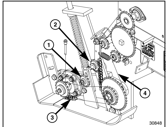
Roller Chains Figure 5-1
