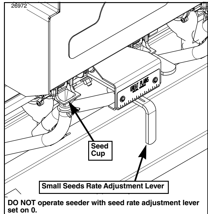
Small Seeds Rate Adjustment Lever Figure 3-10
