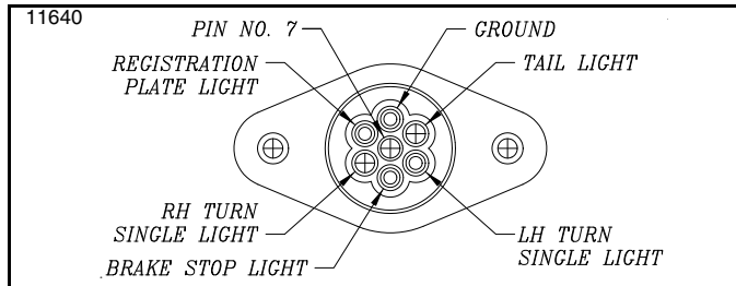
Tractor 7-Pin Electrical Outlet Figure 1-1
