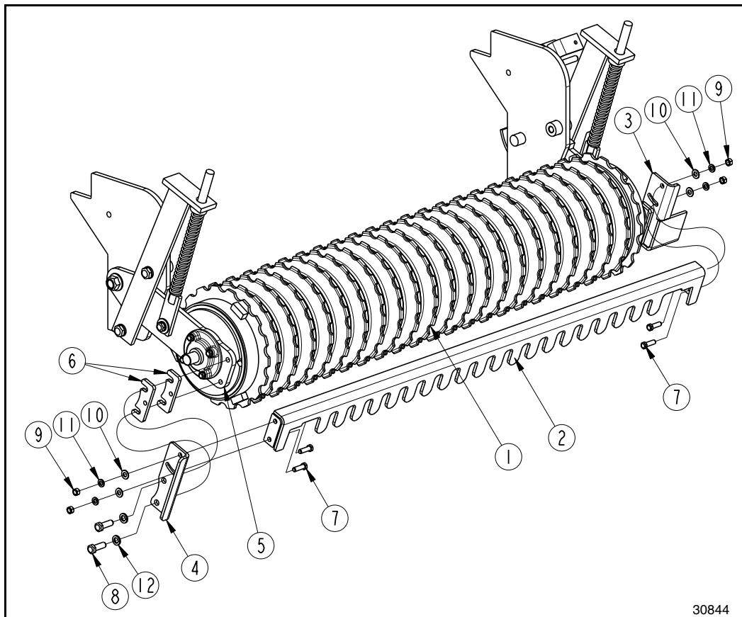
Rear Mud Scraper Installation to Packer Roller Figure 1-4
