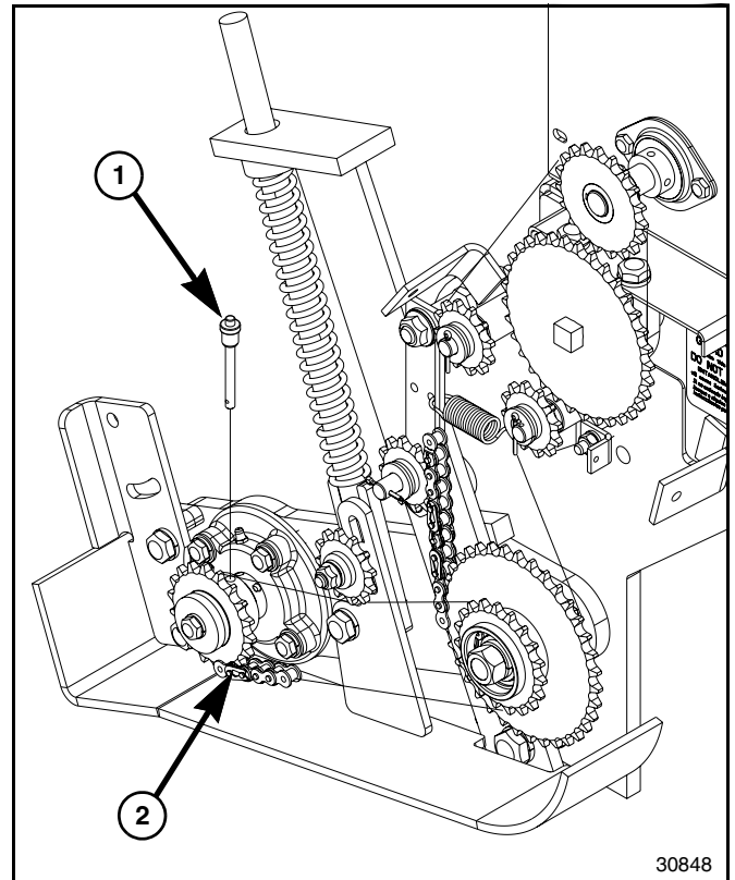
Disengage Drive Chain Figure 3-3
