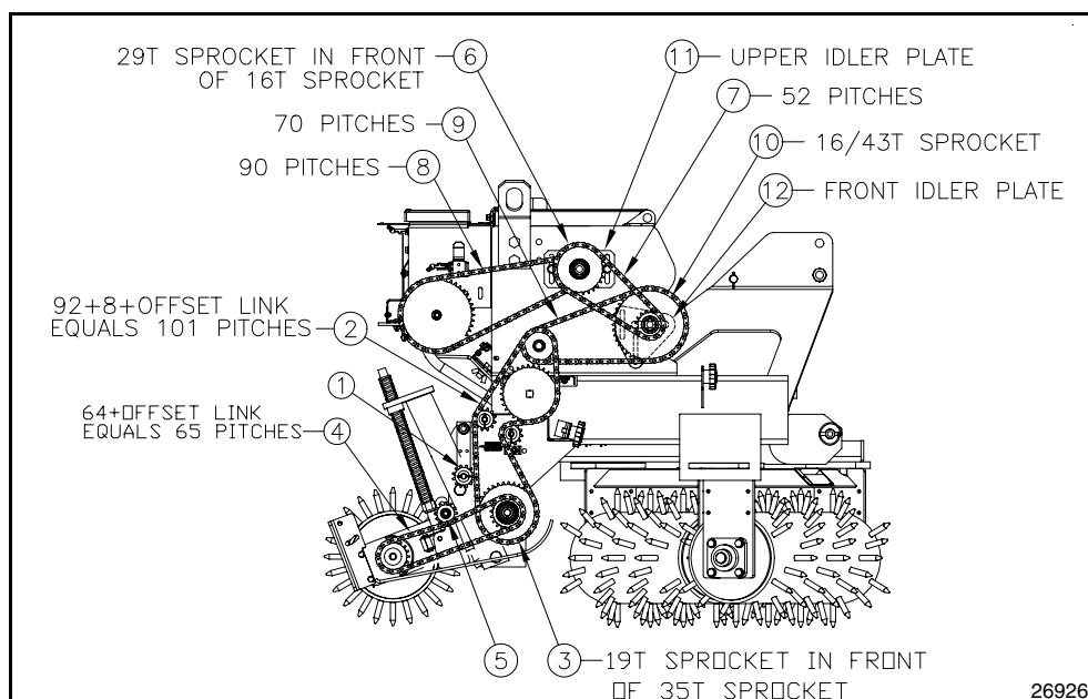
Drive Arrangement With APS Set-Up for High Range Figure 3-8
