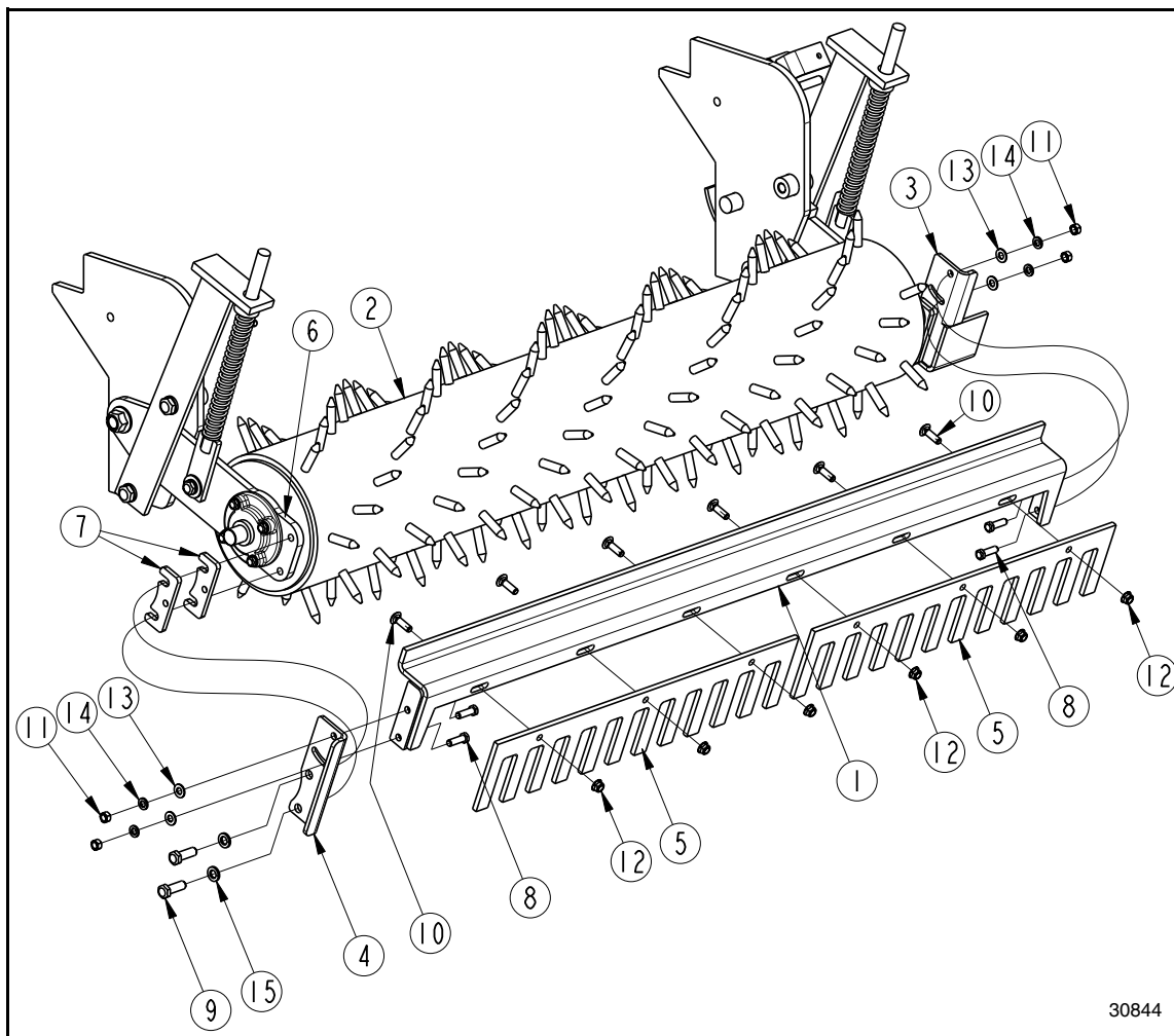
Rear Mud Scraper Installation to Spike Roller Figure 1-5
