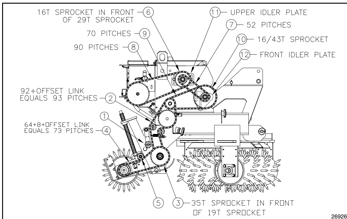
Low Range Sprocket & Chain Arrangement Figure 3-9
