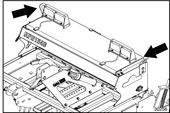
Sling Brackets Figure 1-2
